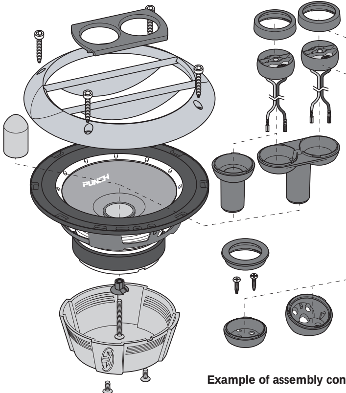
Example of speaker installation
